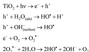
Scheme 1 Reactive radical species generated by \text{TiO}_2 photocatalysis. 85
