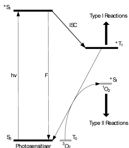
Fig. 4 Jablonski diagram showing energetic transitions from a photo-excited photosensitiser molecule to molecular oxygen ( h\nu = incident visible light energy, F = fluorescence, ISC = intersystem crossing).
