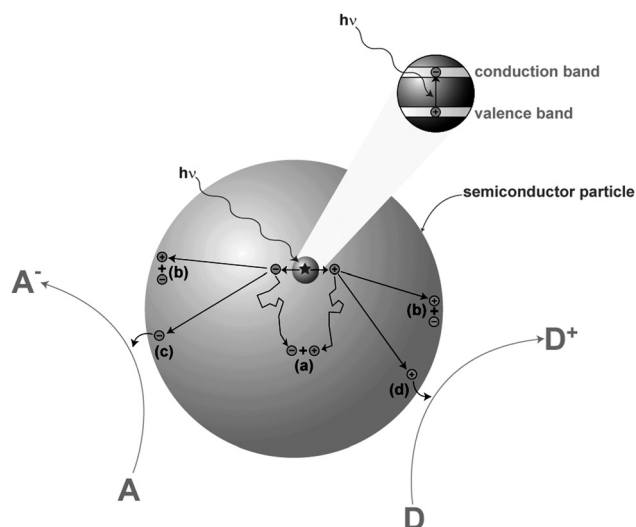
Fig. 5 Photo-excitation processes in \text{TiO}_2 , leading to redox behaviour. (a) Electron and hole recombination in the bulk, (b) electron and hole recombination at the surface, (c) adsorbate reduction at the surface and (d) adsorbate oxidation at the surface.
